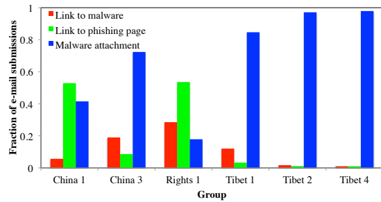
Figure 2: Breakdown of malicious e-mails based on whether they deliver malware as an attachment, refer the use to a link with a malicious file, or attempt to phish data from the user.
