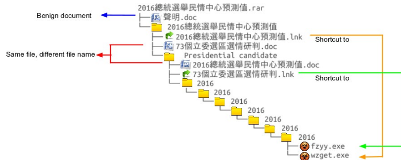
Figure 2: File structure of delivered RAR archive.
