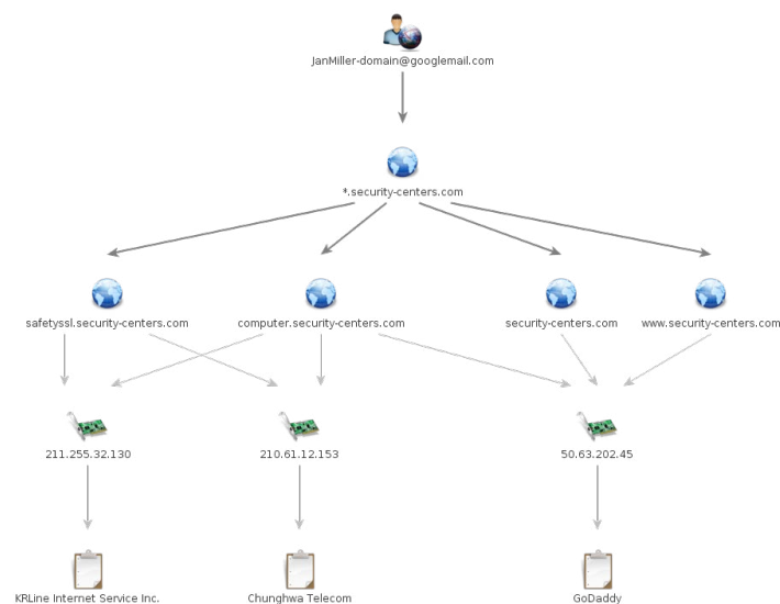
Figure 7: Hosting infrastructure over time for *.security-centers[.]com
